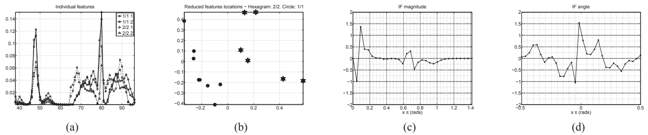
Fig. 2. Analysis of the PLS classification using the combination of scales 1 (see Table 1). (a) Individual features for 2 images 1/1 and 2 images 2/2 in the zones of the |IF| and IF angle only. (b) Coordinate function plots for the 1/1 and 2/2 images. (c) Regression parameter for the |IF| . (d) Regression parameter for the IF angle.
